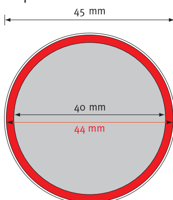
Super-Mini-Clic-Clac-Box
